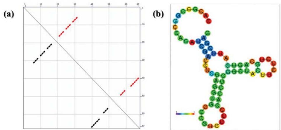
Fig 1. Secondary structure prediction of ATP dependent DNA helicase 3' UTR with calculated \delta G = -11.7 \text{Kcal.mol}^{-1} in this (a) is a graphical representation of each base pairs minimum free energy (MFE) and (b) is secondary structure of the predicted 3'UTR showing the proper formation of stem loop like structures with a typical hammer head like structure.
