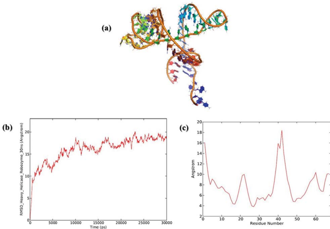
Fig 2. Tertiary structure predictions of ATP dependent DNA helicase putative ribozyme with calculated \delta G = -14.2 \text{ Kcal.mol}^{-1} (b) RMSD and RMSF plots of 30ns MD simulation ATP dependent DNA Helicase putative Ribozyme trajectory. Left panel shows the RMSD and after 6 ns MD simulation the trajectory seems to be stabilized (c) Right panel shows the RMSF indicating that bases 19–22 and 37–42 are highly flexible regions of putative ribozyme.
