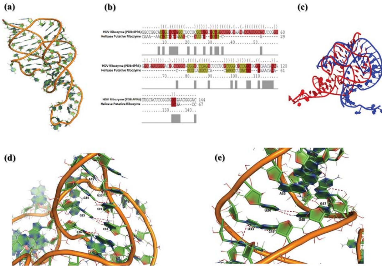
Fig 5. Comparative analysis of Helicase 3' UTR with Hepatitis Delta Virus (HDV) ribozyme (PDB Id: 4PR6). (a) Tertiary structure of HDV Ribozyme (4PR6). (b) Sequence alignment of Helicase 3' UTR and HDV ribozyme. (c) Structural superimposition of HDV ribozyme (4PR6) and Helicase ribozyme where HDV ribozyme is represented in red and Helicase 3' UTR in blue color respectively. (d) Canonical base pairing are observed during the MD simulation of Helicase 3' UTR. In this we have shown the base pairing between G25-C18, A23-U20, which are regular Watson-crick base pairings. (e) Non-canonical base pairing which are normally seen in RNA structures are also observed during Helicase 3' UTR MD simulations. In this we have shown base-pairings between A35-G47, U34-U48, and U33-C49. Apart from these Hoogsteen base pairings are also seen.
