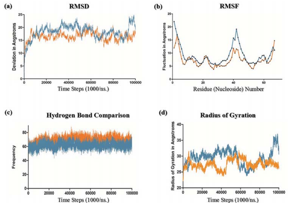
Fig 4. MD simulation event analysis comparison of Helicase 3' UTR 100ns MD simulations in presence and in absence of MgCl 2 . In all the images events of Helicase 3' UTR is represented in light blue color and the same events in presence of MgCl 2 is represented in orange colour (a) RMS deviation is more stabilized in presence of MgCl 2 than in the absence of salt. (b) RMS fluctuations are recorded similarly when compared with the presence of salt showing the lesser fluctuations than in its absence. (c) No. of. Intra molecular Hydrogen bond analysis suggests that in presence of salt RNA is more stable than in the absence of it. (d) Radius of gyration analysis also shows more stable structural movements in presence of salt rather than in its absence. Thus our simulations in presence of MgCl 2 shows more favorable environment rather than in the absence of it.
