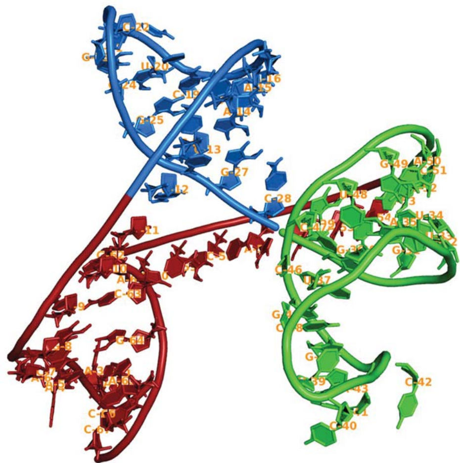
Fig 3. Rigid domains of Putative Ribozyme identified using RNA Normal Mode analysis indicated with red and blue colors, flexible domains are denoted in green color.
